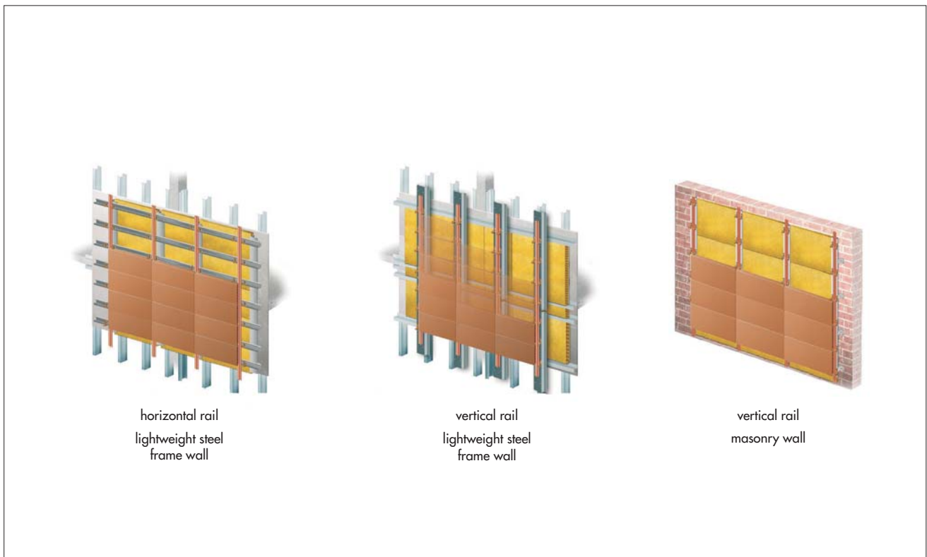
Figure 1 General arrangement of support systems
