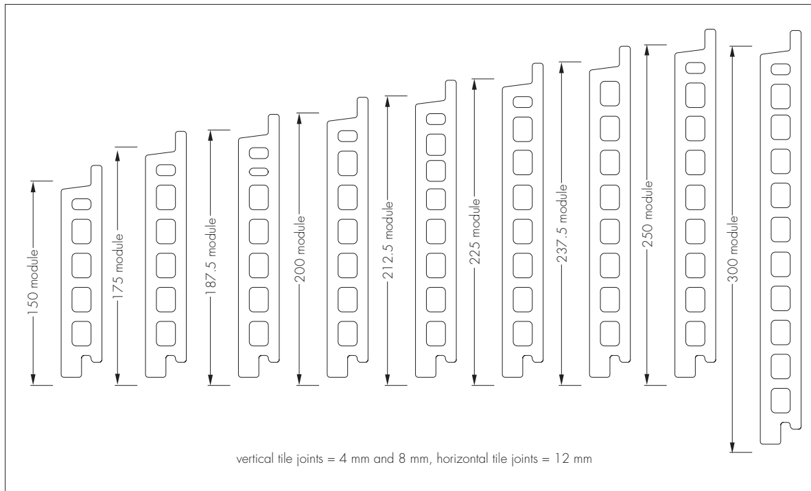
Figure 2 Tile modules (dimensions in mm)
